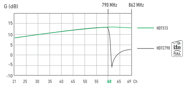
Gain diagrams
